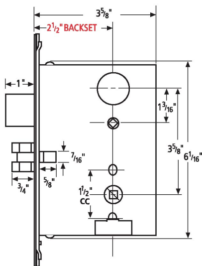
2½" Backset Lock
