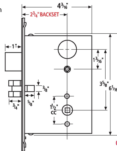
2¾" Backset Lock
