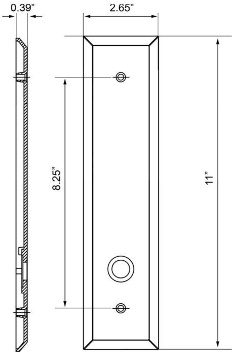
Side View
