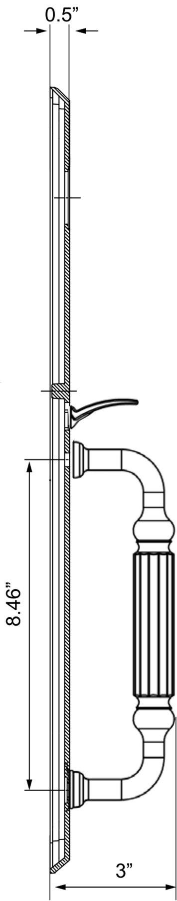
Side View
