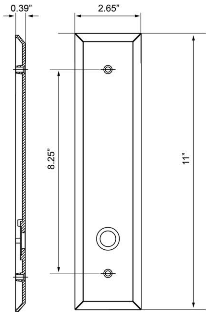
Side View
