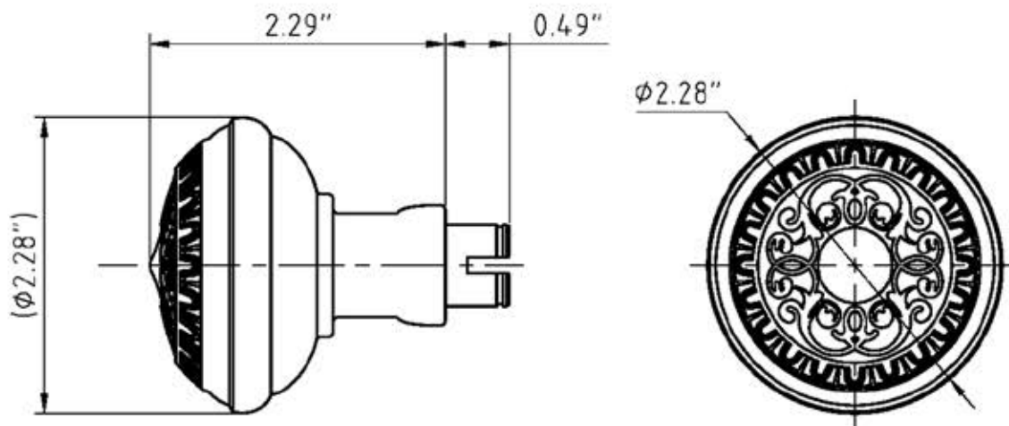
Side View
