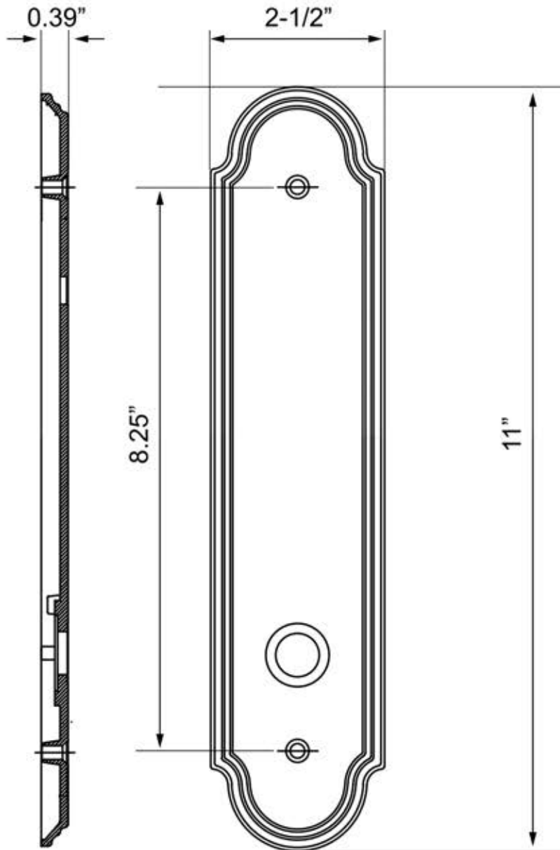
Side View
