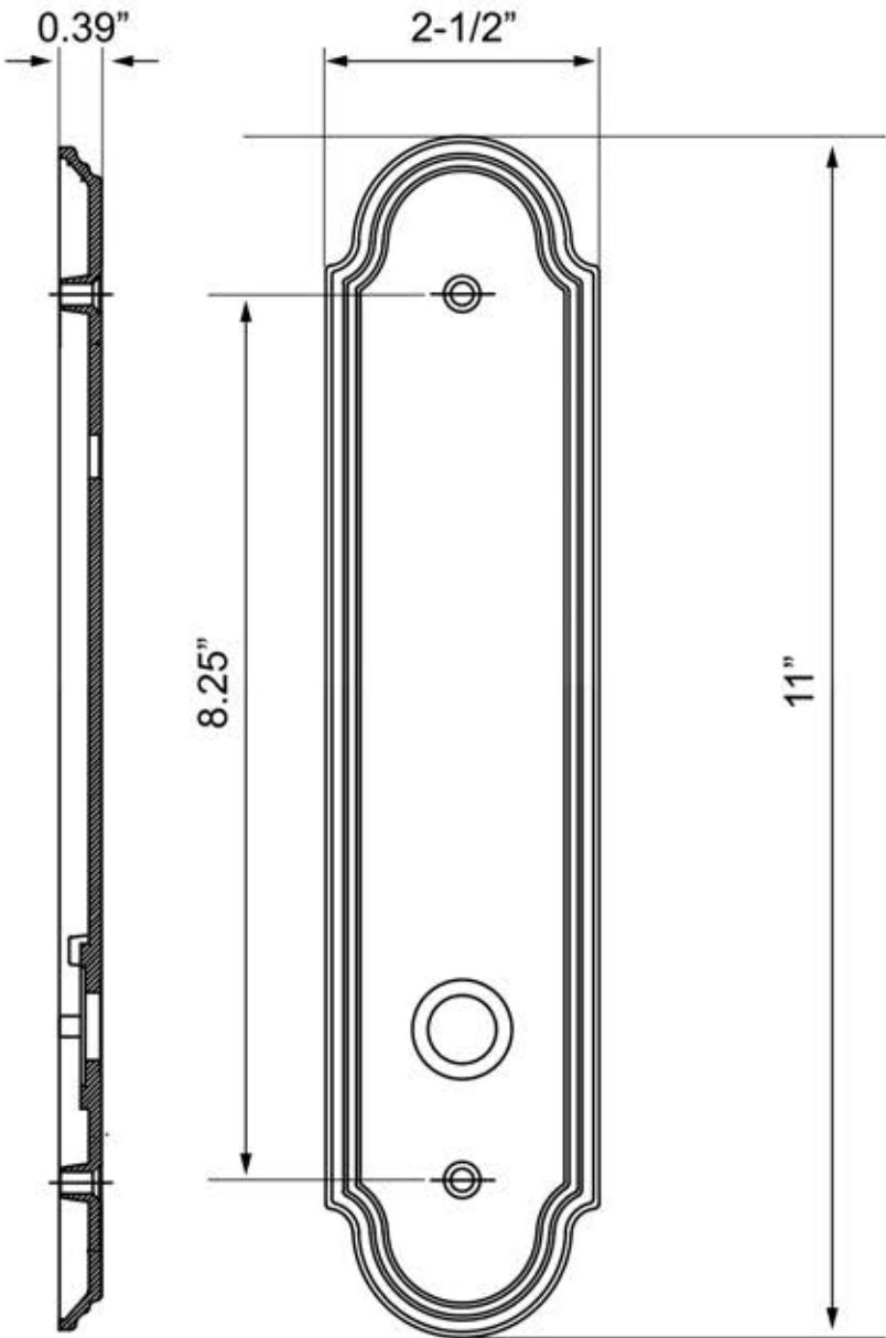
Side View
