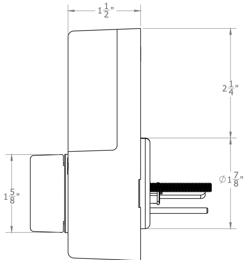
SIDE VIEW
