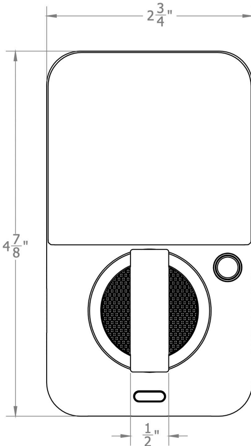
FRONT VIEW
