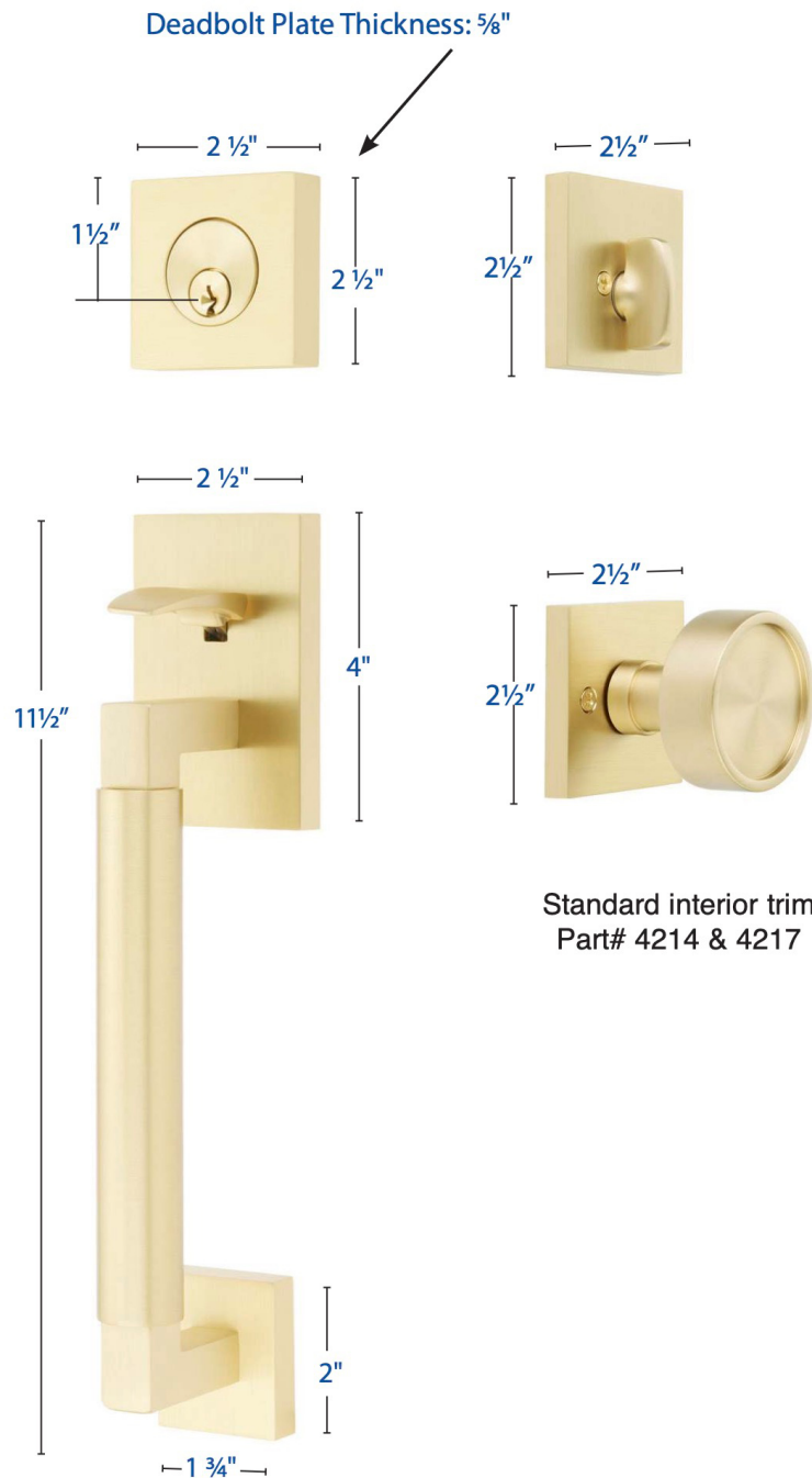
Hercules Sectional Smooth/Knurled Styles Part # 4214 & 4217
