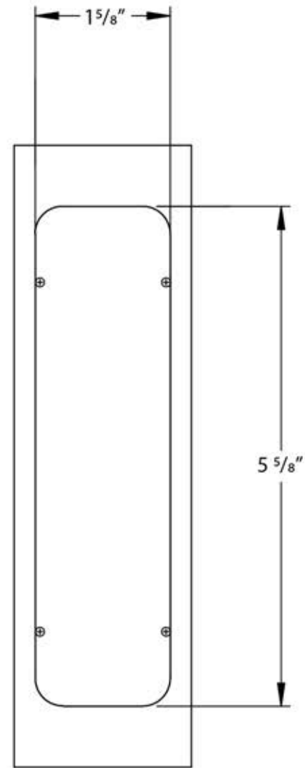
BACK VIEW
