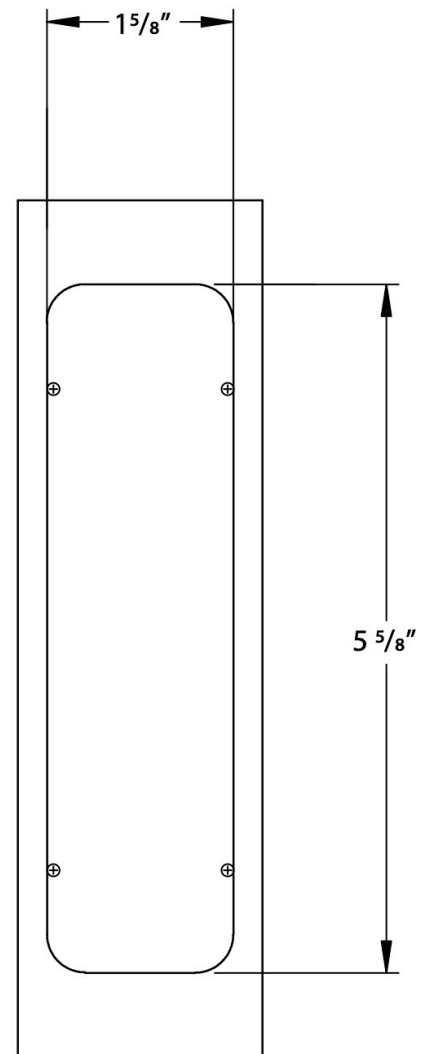
BACK VIEW
