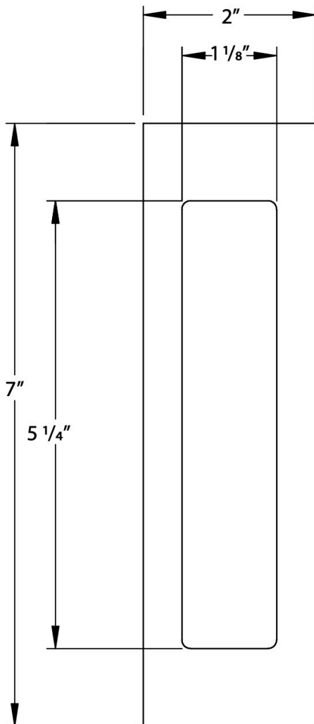
FRONT VIEW
