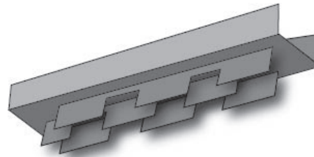
Optional: Notched Fins - Suffix "NF" Allows air flow while restricting light.
