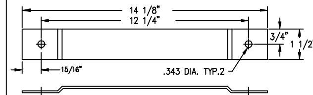
GUIDE PLATE
