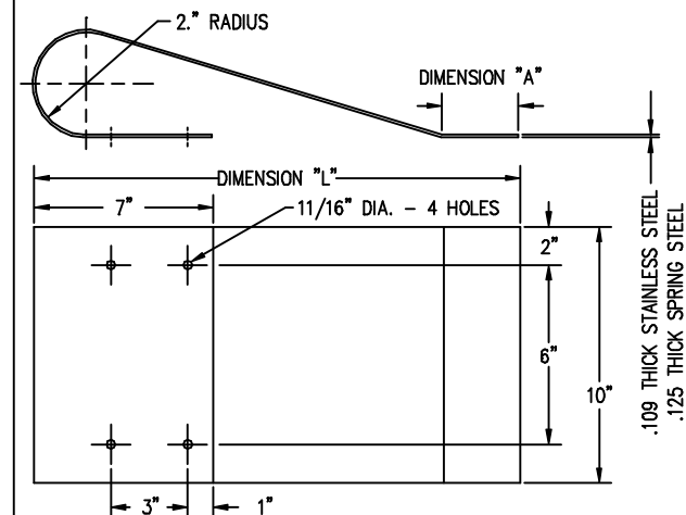
BUMPER
